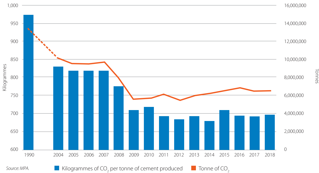
6.3a: Carbon dioxide emissions from UK cement production plants
