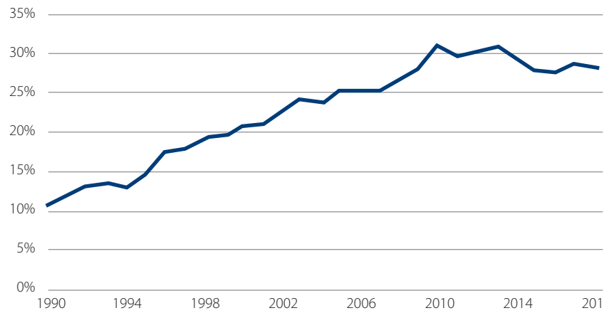
6.1a: Recycled and secondary materials in total aggregates sales in Great Britain, 1990-2018
