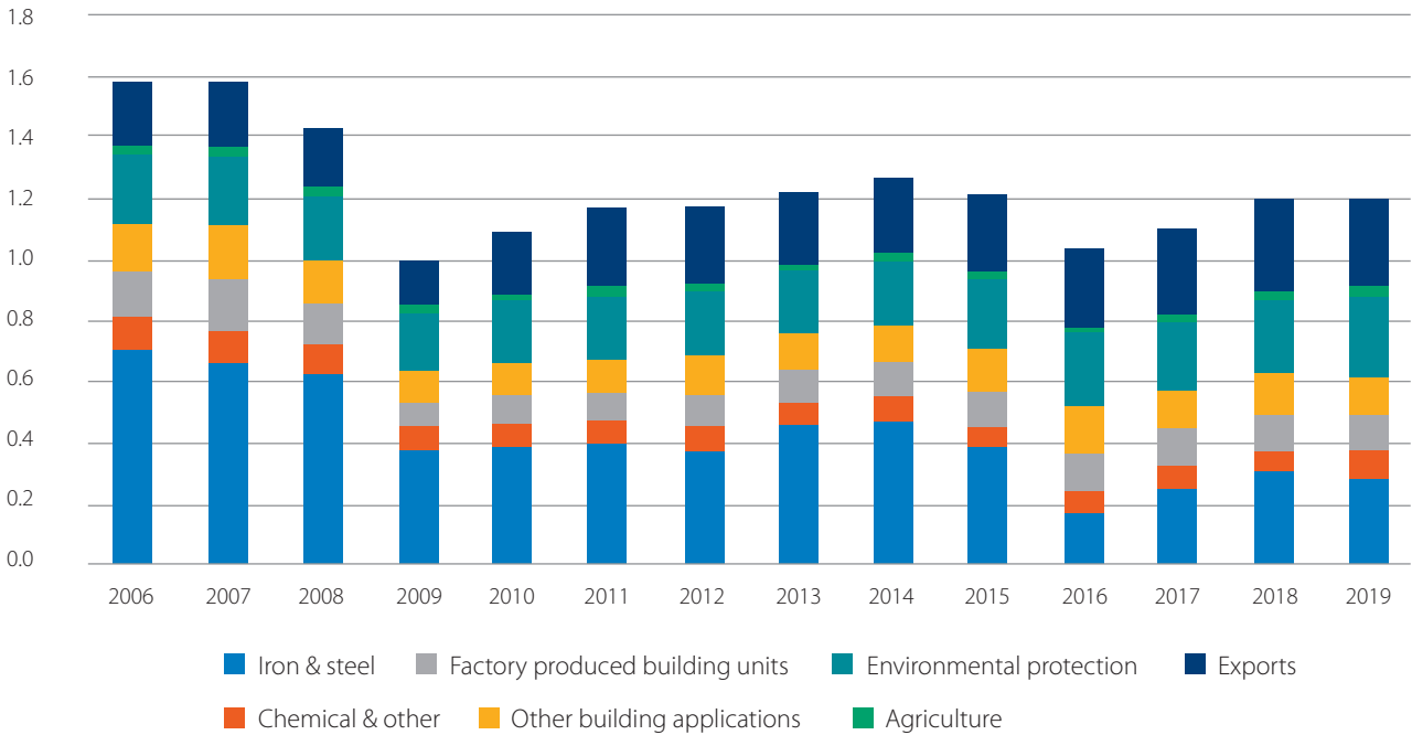
3.5a: Industrial lime sales by end-usage in Great Britain, 2006-19 (Million tonnes)
